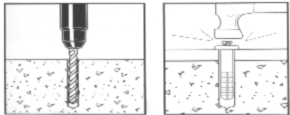
ST-357 Flat Head NYLON NAIL ANCHOR Application Concrete, Solid Brick, Stone Material Body:Nylon or PE Nail:Steel,1010-1018,withZinc,Yellow Zinc Plated
