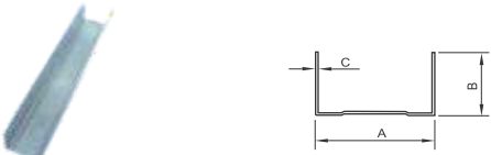
LP1007 A(mm):28 B(mm):27 C(mm):0.4,0.5
