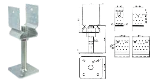
LP3001 T:4 AxB(mm):61x60,71x80,81x80,91x100,101x100, 121x100,121x120,141x120
