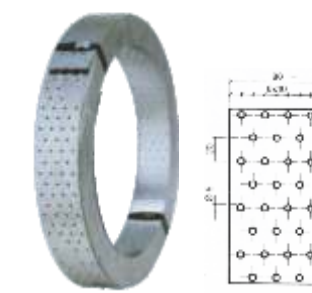
ST-J-BP-8 60X2.0X10000mm 60X2.0X25000mm
