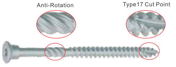
ST-1912 CHIPBOARD SCREW Torx
