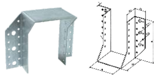
LP3008 T:2 AxB(mm):51x100,81x80,81x100,81x120,81x140, 101x100,101x120,101x140,121x120, 121x140,141x160,161x200
