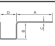
LP1024 A(mm):27 B(mm):12.5 C(mm):0.45 D(mm):12.5
