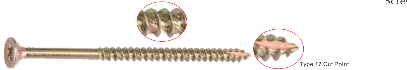
ST-18001 CHIPBOARD SCREW Countersunk Head Pozidriv
