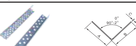
LP1014 A(mm):23,25,28,30,51 B(mm):23,25,28,30,51 C(mm):0.4,0.45,0.5
