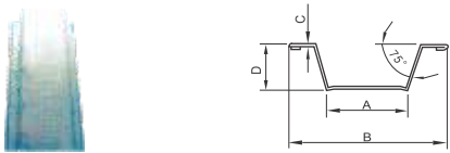
LP1001 A(mm):30,32,35,50 B(mm):68,73,80,85,88 C(mm):0.45,0.5 D(mm):10,20,22,25,35,38
