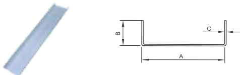
LP1004 A(mm):30,38,45,50,60 B(mm):10,11,12,13,15,25,27 C(mm):0.45,0.5,0.6,0.7,.08,0.9,1,1.2
