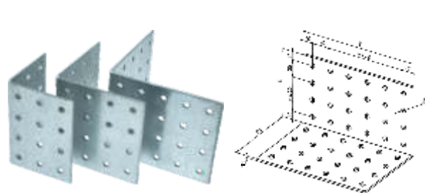
LP3011 T:2 AxBxC(mm): 40x40x40,40x60x60,60x80x80,60x100x100, 80x80x60,80x80x80,80x80x100,80x120x120, 100x120x120,100x140x140,120x140x140, 140x160x160,160x200x200,200x240x240
