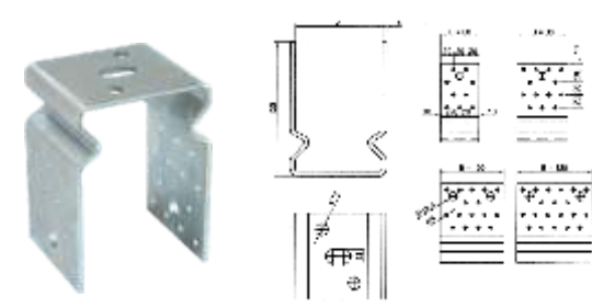
LP3006 T:4 AxB(mm):61x60,71x80,81x80,91x100,101x100, 121x100,121x120,141x120
