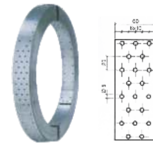
ST-J-BP-7 40X2.0X10000mm 40X2.0X25000mm
