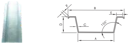
LP1002 A(mm):30,32,35,50 B(mm):68,73,80,85,88 E(mm):9 C(mm):0.45,0.5 D(mm):10,20,22,25,35,38 F(mm):3
