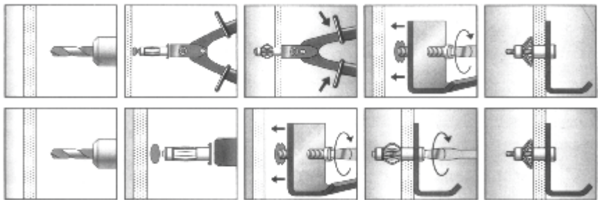
ST-17045-A HOLLOW WALL ANCHOR SETTING TOOL
