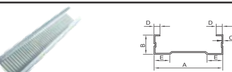
LP1022 A(mm):35 B(mm):11 D(mm):3 E(mm):8 C(mm):0.3,0.4,0.45,0.5
