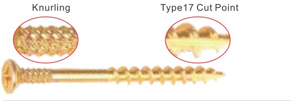
ST-1909 CHIPBOARD SCREW Countersunk Head With Ribs Uner Countersunk Pozi,Phillips
