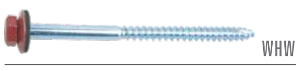
ST-041 WOOD SCREW DIN 571 Wood Screw(Full Thread) Hex Head With Steel & Rubber Washer, Tape17 Head Painted
