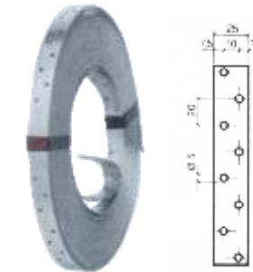
ST-J-BP-2 25X2.0X10000mm 25X2.0X25000mm
